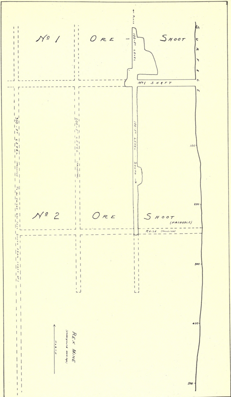
Underground Plan, Rex Mine
