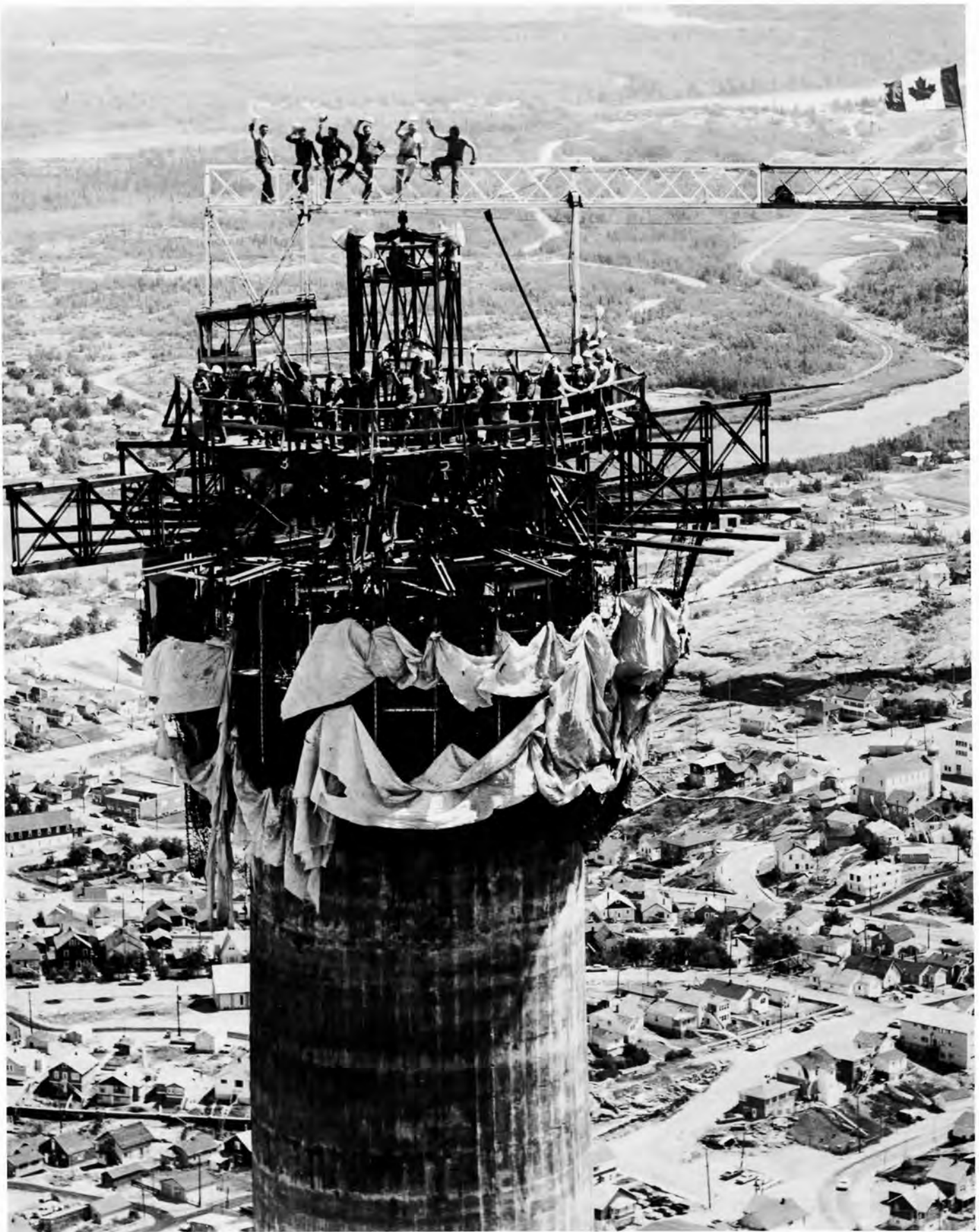
Topping off the 825 foot stack on Company property — July 1973. (HBM&S)
